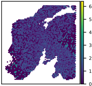
SNU24A SLC2A13 expression Moran's I = 0.09
