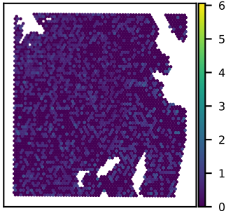
SNU51A HMGXB4 expression Moran's I = 0.01
