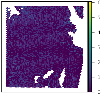
SNU51A TMEFF2 expression Moran's I = 0.07
