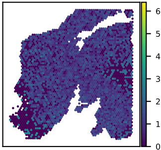
SNU24A CDC34 expression Moran's I = 0.06
