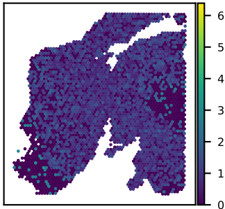
SNU24A PIK3C3 expression Moran's I = 0.06
