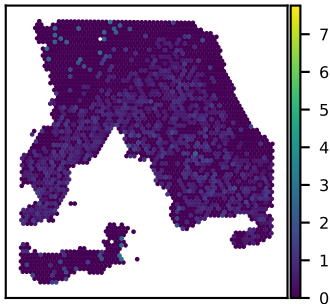
SNU18A C3AR1 expression Moran's I = 0.08
