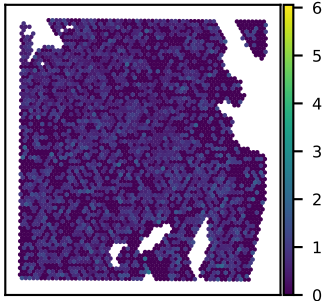
SNU51A BICRA expression Moran's I = 0.03
