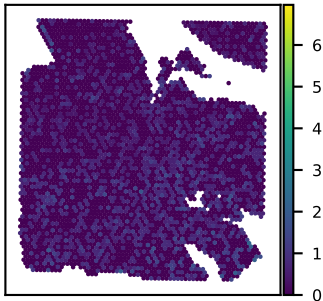
SNU24B RCSD1 expression Moran's I = 0.03
