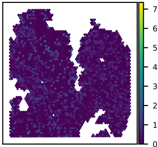
SNU27B HDAC9 expression Moran's I = 0.05
