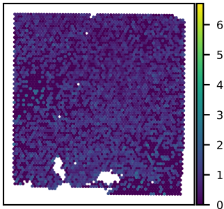
SNU43A FADS1 expression Moran's I = 0.04
