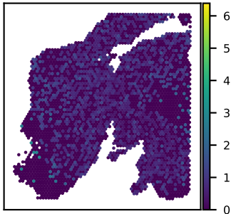
SNU24A NR1D1 expression Moran's I = 0.04
