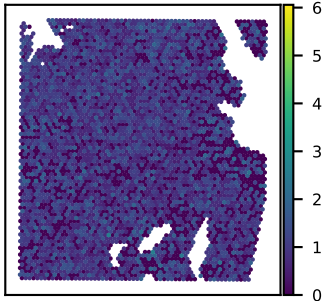
SNU51A HADHB expression Moran's I = 0.03
