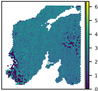
SNU24A NRCAM expression Moran's I = 0.26
