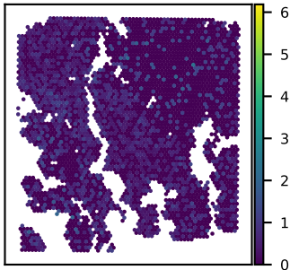
SNU16B RNF113A expression Moran's I = 0.04
