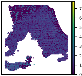
SNU18A CHMP3 expression Moran's I = 0.16
