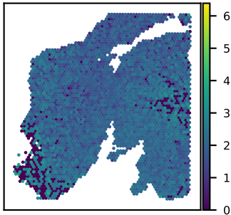
SNU24A CNTN1 expression Moran's I = 0.09
