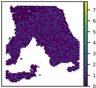
SNU18A WDR60 expression Moran's I = 0.03
