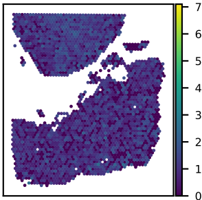
SNU25A CTNNBIP1 expression Moran's I = 0.10
