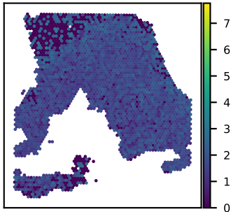
SNU18A CHMP2A expression Moran's I = 0.14
