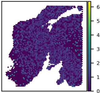
SNU24A RBM27 expression Moran's I = 0.05
