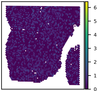
SNU25B C16orf87 expression Moran's I = 0.01
