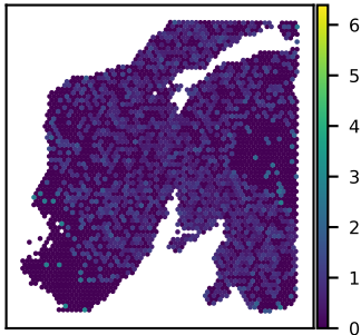
SNU24A C11orf95 expression Moran's I = 0.05
