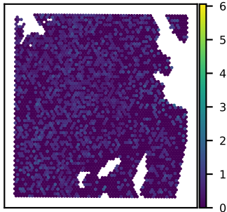
SNU51A SH3D19 expression Moran's I = 0.03
