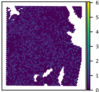
SNU51A STK32B expression Moran's I = 0.02
