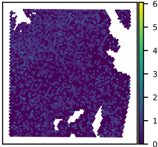
SNU51A OSBPL3 expression Moran's I = 0.05
