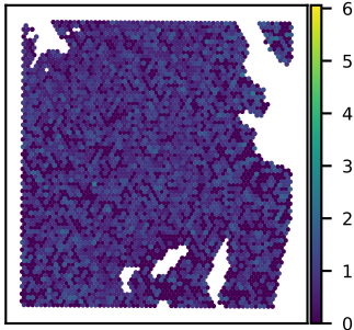
SNU51A BCAP29 expression Moran's I = 0.03
