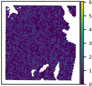
SNU51A NCKAP5L expression Moran's I = 0.00
