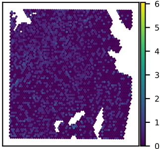
SNU51A CSR2 expression Moran's I = 0.03
