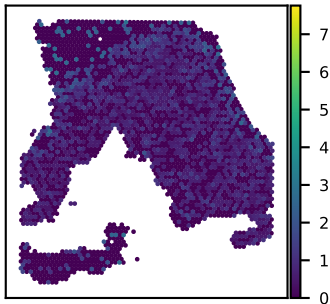
SNU18A C8orf76 expression Moran's I = 0.08
