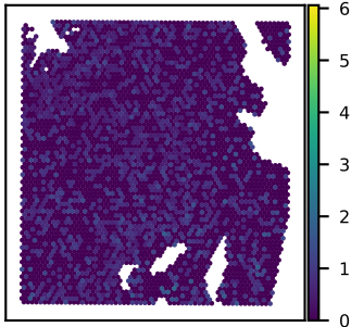
SNU51A TMEM41A expression Moran's I = 0.01
