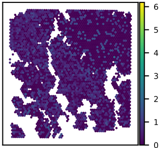
SNU16B KCNA2 expression Moran's I = 0.05
