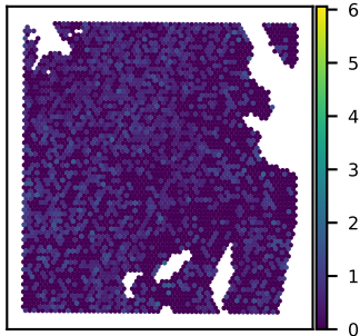
SNU51A PAPSS2 expression Moran's I = 0.05
