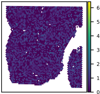
SNU25B SH3BGR expression Moran's I = 0.01
