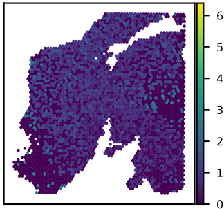
SNU24A TBC1D12 expression Moran's I = 0.10
