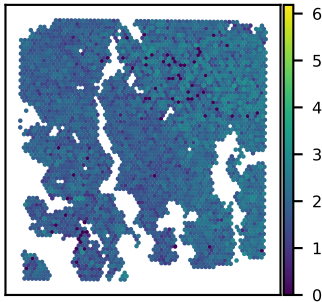
SNU16B SNRNP70 expression Moran's I = 0.16
