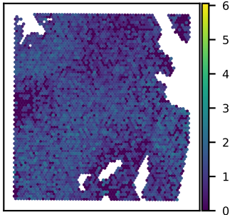
SNU51A SPRY4 expression Moran's I = 0.22
