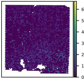
SNU43A MAPK8IP2 expression Moran's I = 0.08
