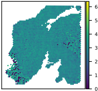
SNU24A PABPC1 expression Moran's I = 0.05
