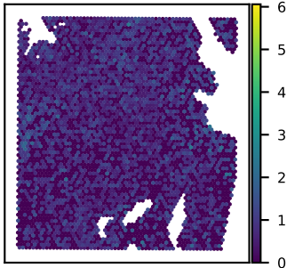
SNU51A STOM expression Moran's I = 0.04
