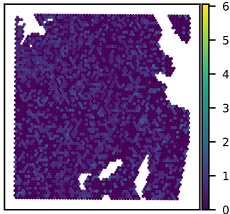
SNU51A UGGT2 expression Moran's I = 0.03
