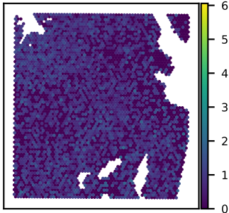
SNU51A HSPB6 expression Moran's I = 0.05
