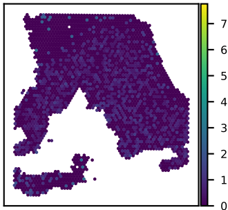
SNU18A DHRS12 expression Moran's I = 0.03
