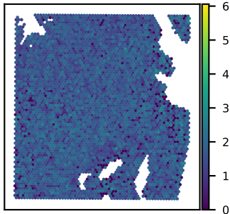
SNU51A NDUFS6 expression Moran's I = 0.02
