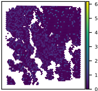
SNU16B STXBP5L expression Moran's I = 0.03
