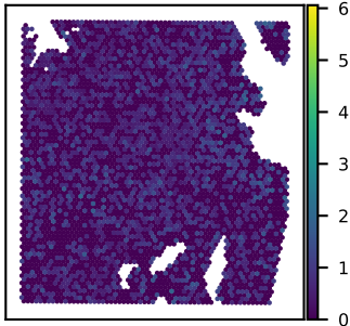
SNU51A FAM184A expression Moran's I = 0.03
