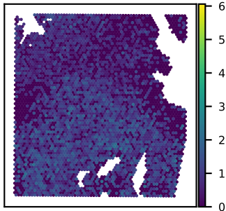
SNU51A NKAIN1 expression Moran's I = 0.23
