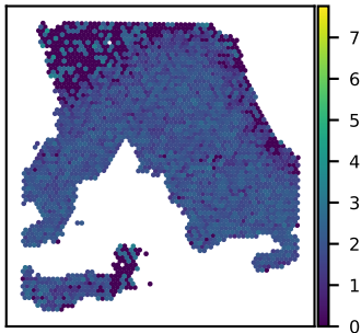
SNU18A PPP1CB expression Moran's I = 0.31
