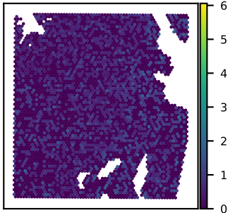
SNU51A RAB40C expression Moran's I = 0.01
