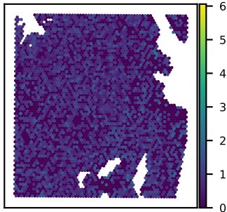
SNU51A DENND4B expression Moran's I = 0.01
