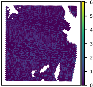
SNU51A C1orf112 expression Moran's I = 0.03
